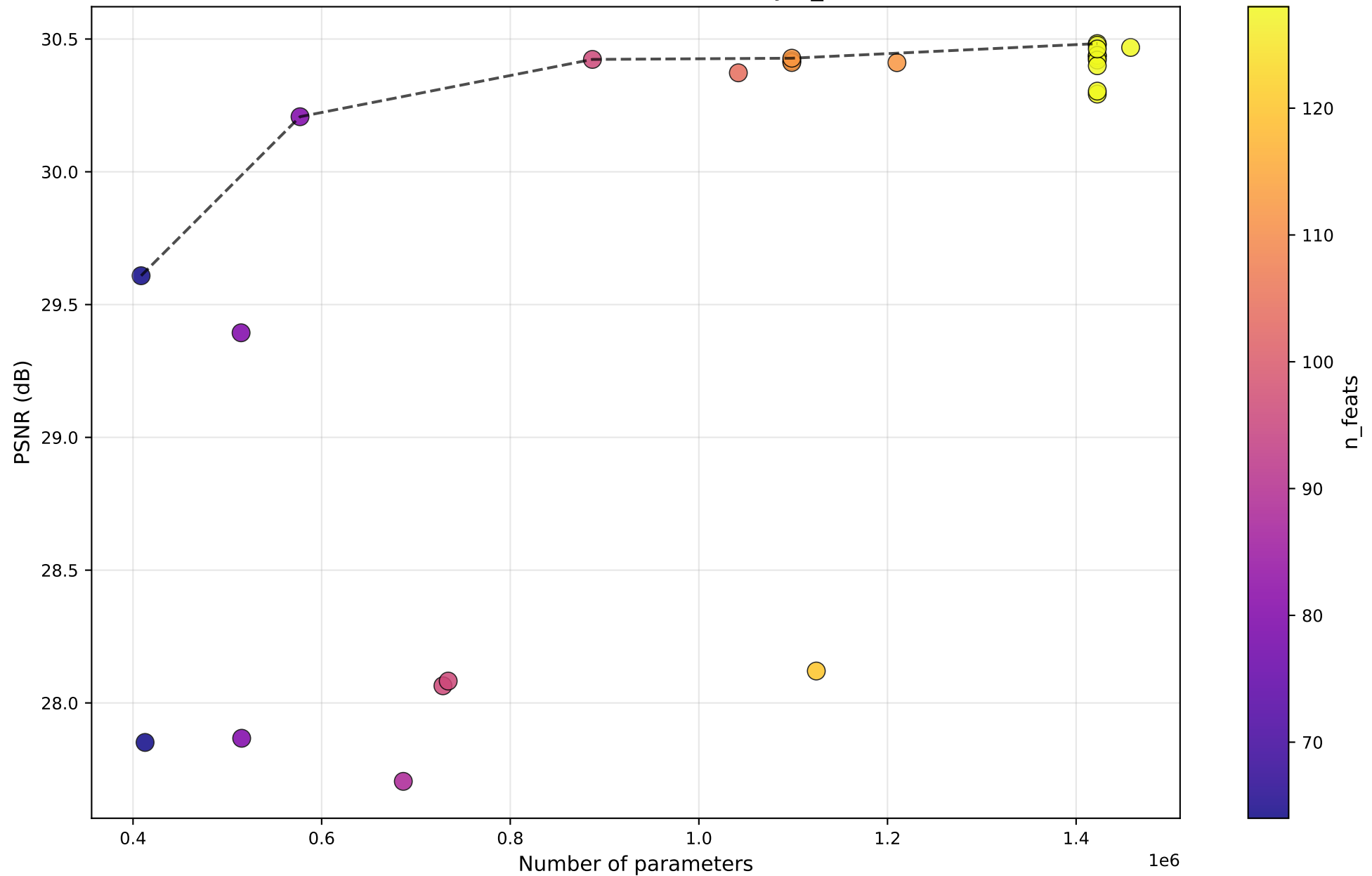
PSNR vs #Params — SwinT — by n_feats
